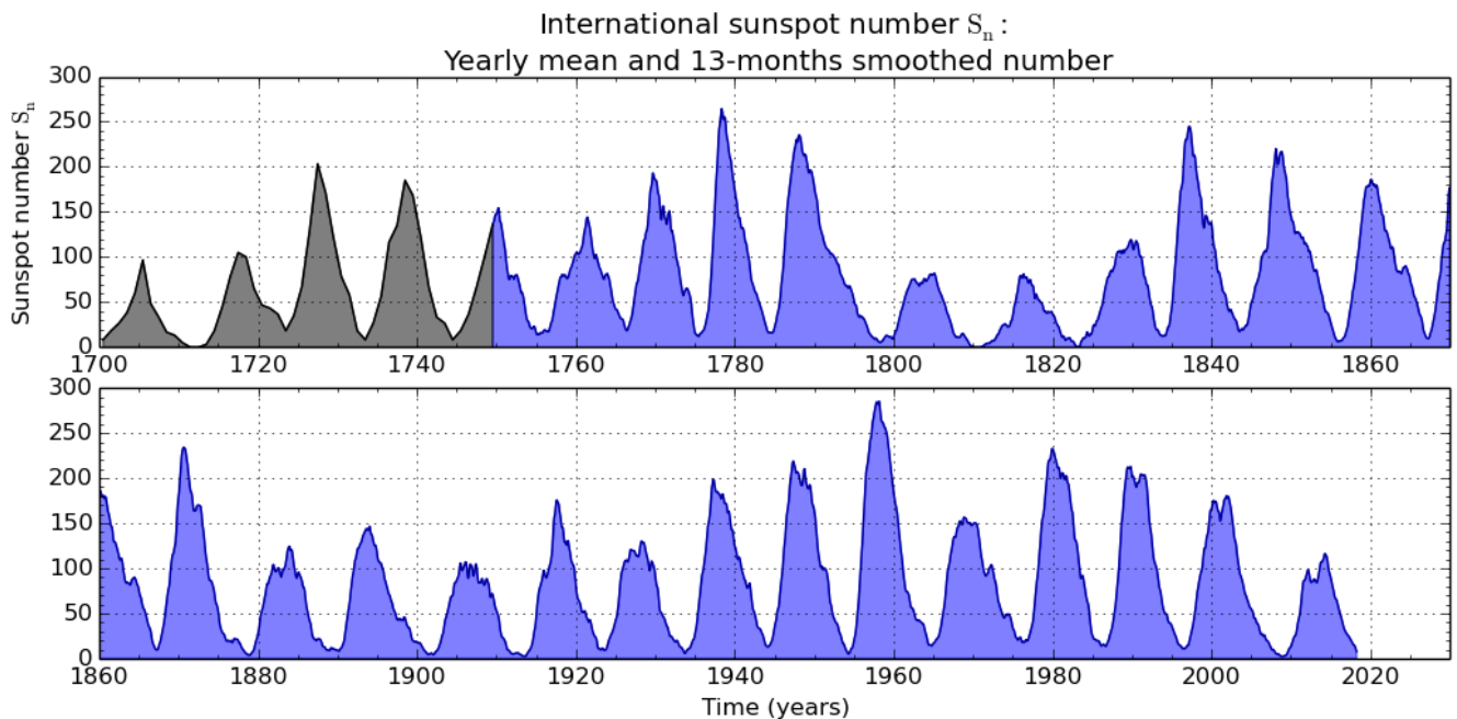
SILSO graphics ( http://sidc.be/silso ) Royal Observatory of Belgium 2018 November 1
